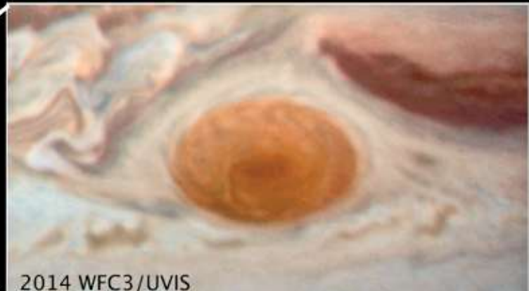
2014 WFC3/UVIS
