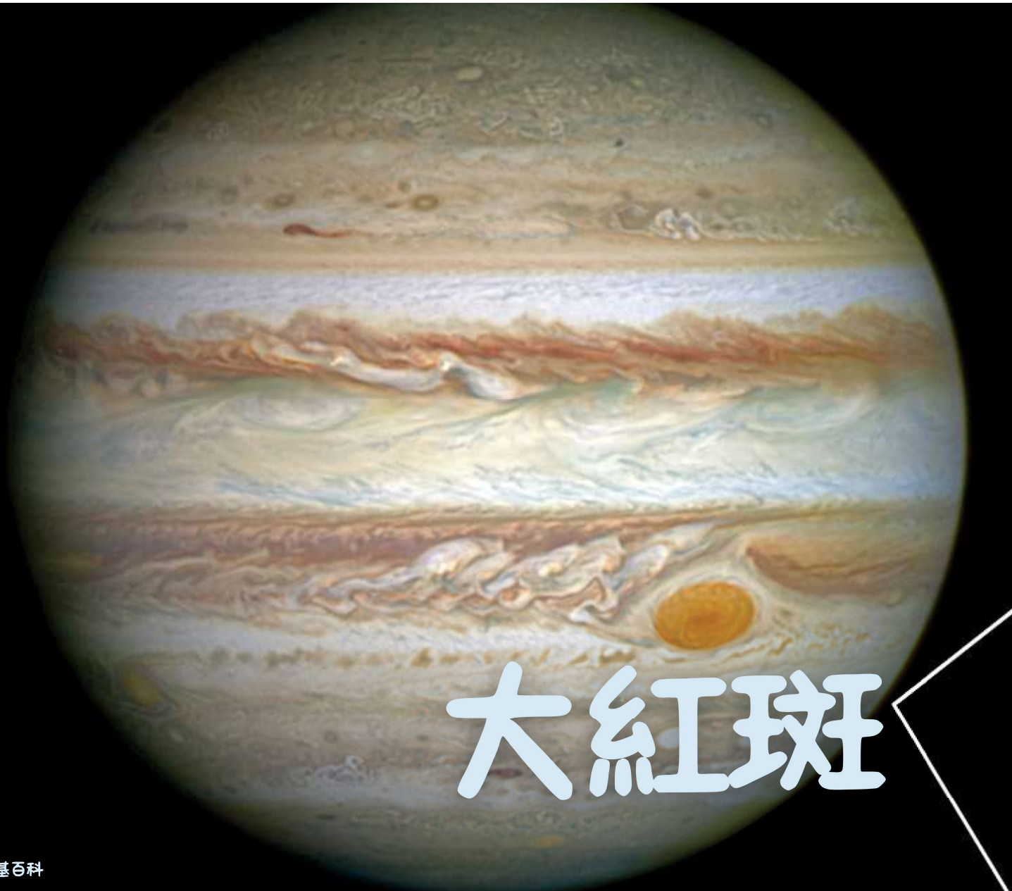
1995 WFC2
